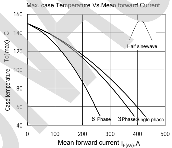
Fig.4 Max Case Temperature Vs. Mean Forward Current
