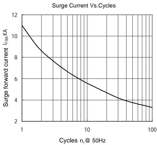
Fig.7 Surge Current Vs.Cycles Curve
