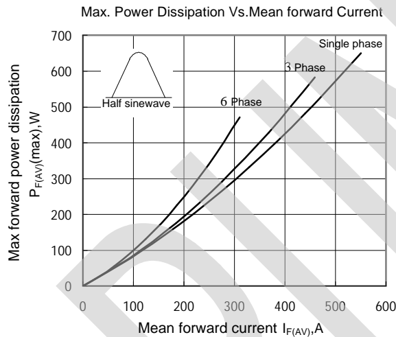
Fig.3 Max Power Dissipation Vs. Mean Forward Current
