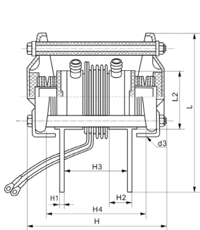
SS11, SS12 water cooling heatsink
