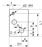
SS13, SS14 conductor plate
