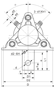
SS11, SS12 water cooling heatsink
