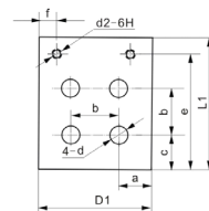
SS15, SS16 conductor plate
