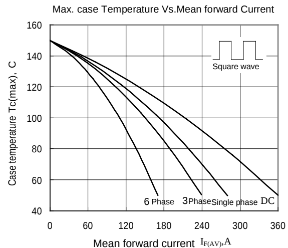
Fig.6 Max Case Temperature Vs. Mean Forward Current
