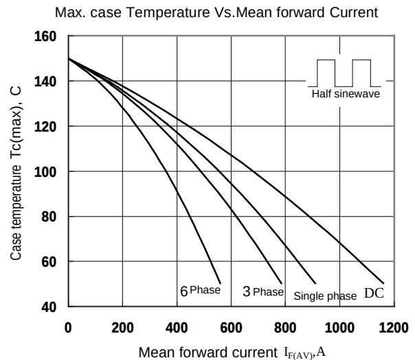
Fig.6 Max Case Temperature Vs. Mean Forward Current
