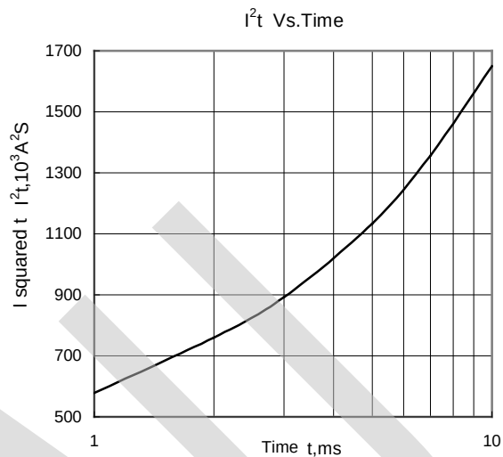
Fig.8 I^2t Vs.Time
