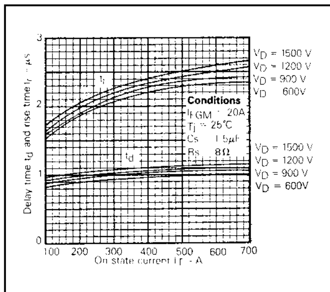
Fig.14 Delay time and rise time vs on-state current
