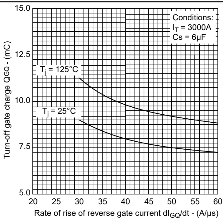
Fig.27 Turn-off gate charge vs rate of rise of reverse gate current
