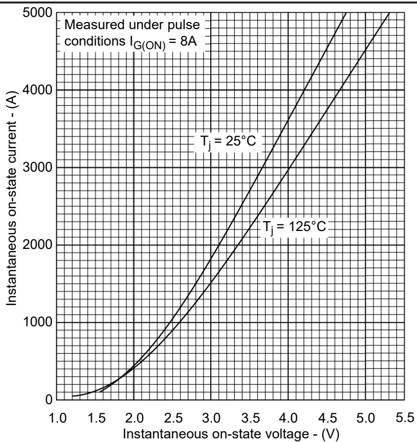
Fig.2 On-state characteristics
