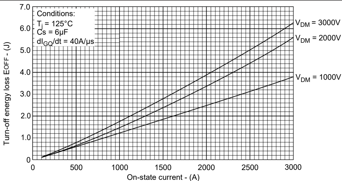
Fig.17 Turn-off energy vs on-state current
