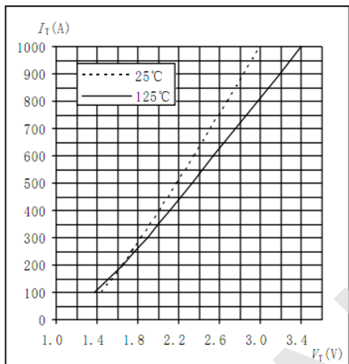
Fig.1 On-state Volt-ampere Characteristic Curve
