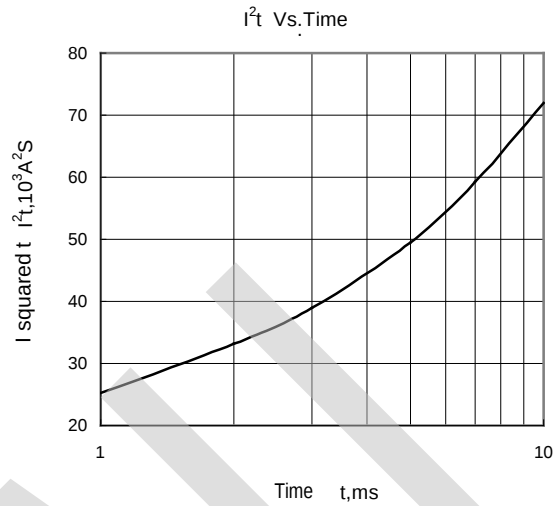
Fig.8 I^2t Vs.Time
