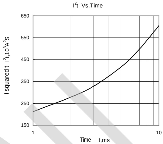
Fig.8 I^2t Vs.Time
