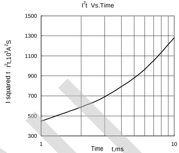
Fig.8 I^2t Vs.Time
