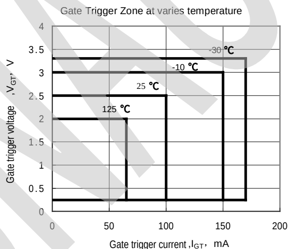
Fig.10 Gate Trigger Characteristic Curve
