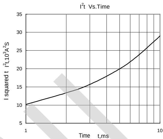
Fig.8 I^2t Vs.Time
