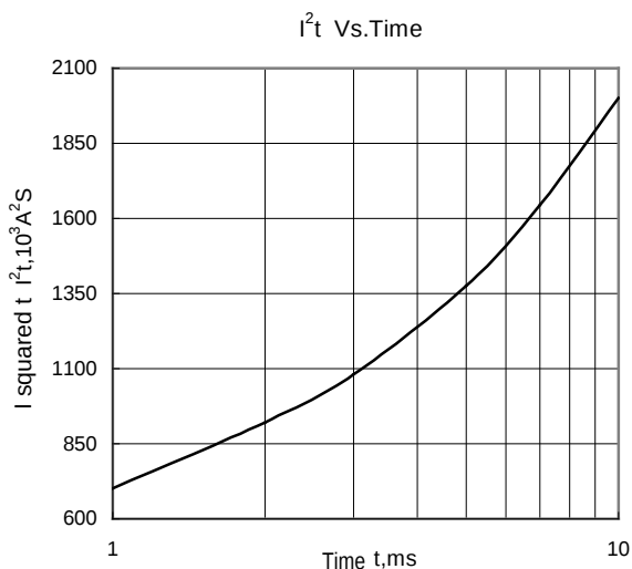
Fig.8 I^2t Vs.Time
