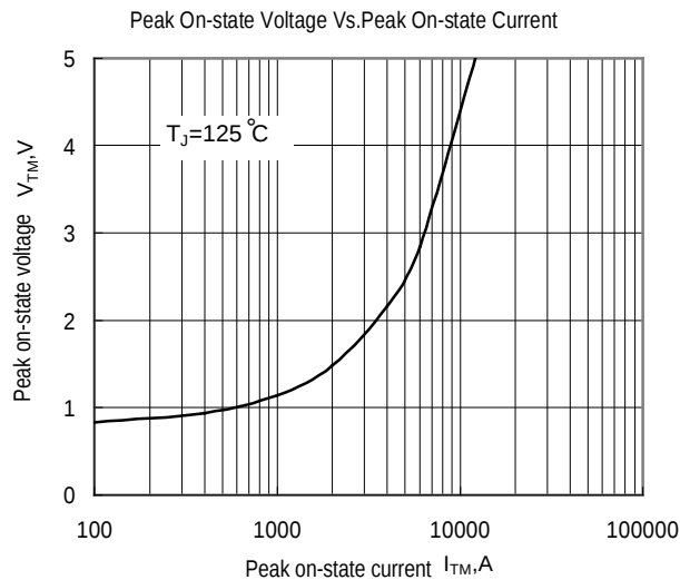
Fig.1 On-state Volt-ampere Characteristic
