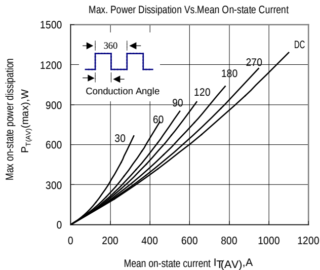
Fig.5 Max Power Dissipation Vs. Mean On-state Current
