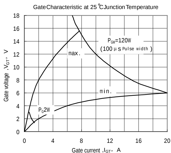
Fig.9 Gate Power Graph
