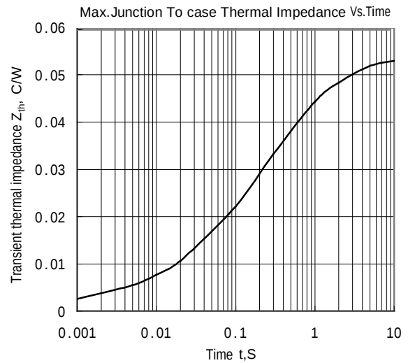
Fig.2 Transient Thermal Impedance of Junction to Case
