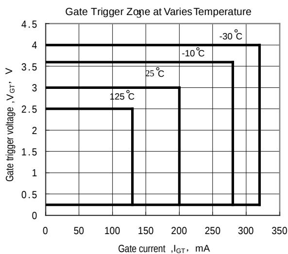
Fig.10 Gate Trigger Characteristic Graph
