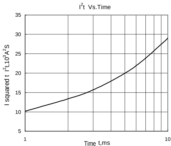
Fig.8 I^2t Vs.Time
