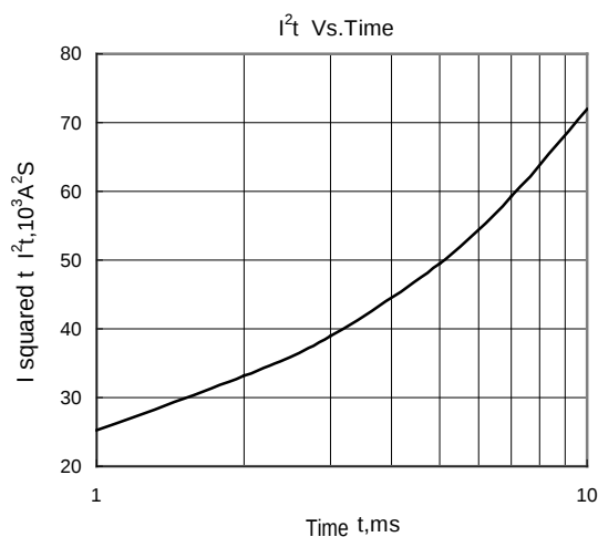
Fig.8 I^2t Vs.Time
