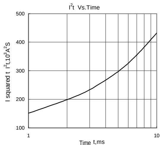
Fig.8 I^2t Vs.Time
