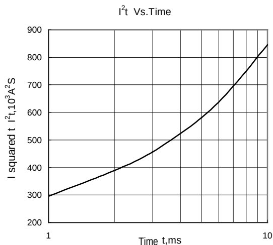
Fig.8 I^2t Vs.Time
