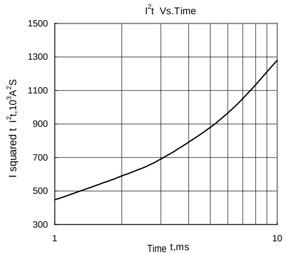
Fig.8 I^2t Vs.Time
