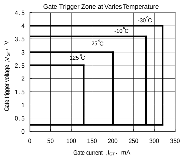
Fig.10 Gate trigger characteristic graph
