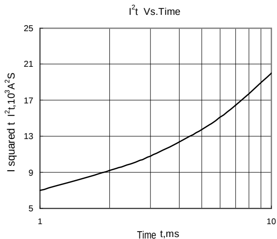
Fig.8 I^2t Vs.Time
