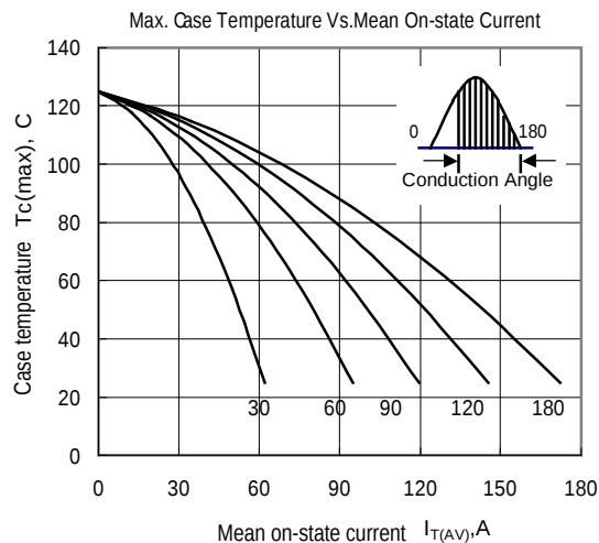
Fig.4 Max case Temperature Vs. Mean on-state Current
